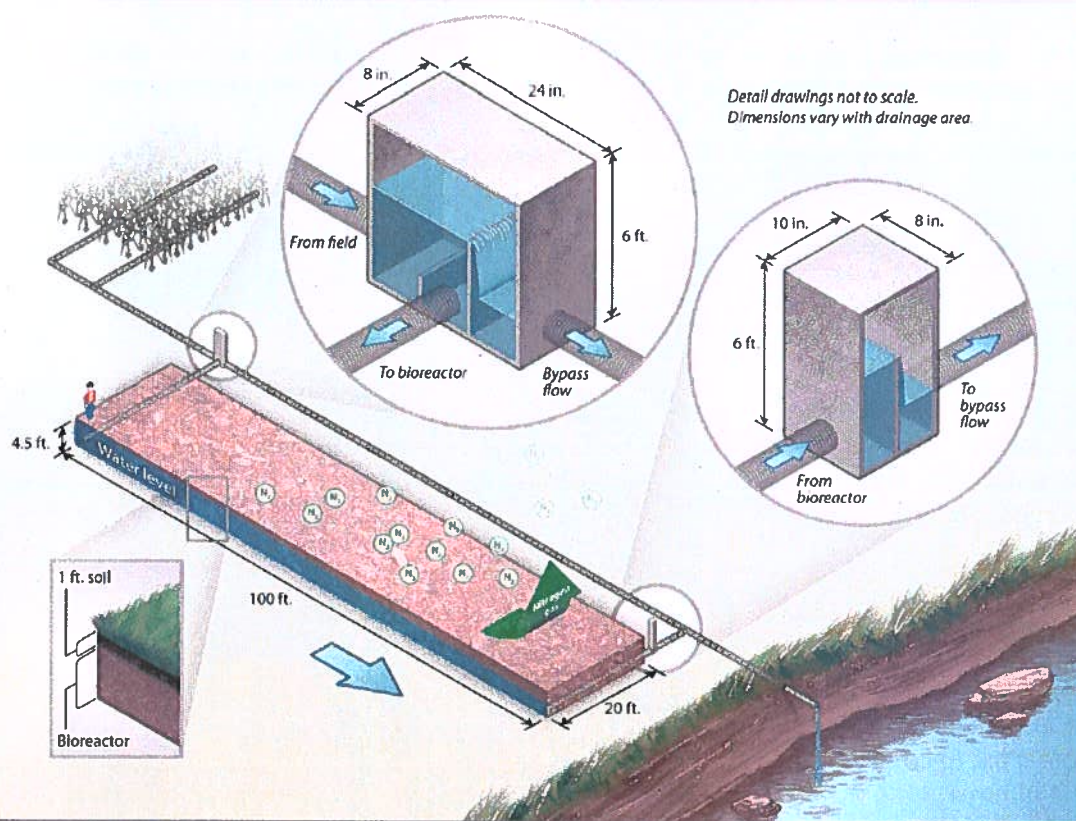
Illustration of a denitrifying bioreactor.
